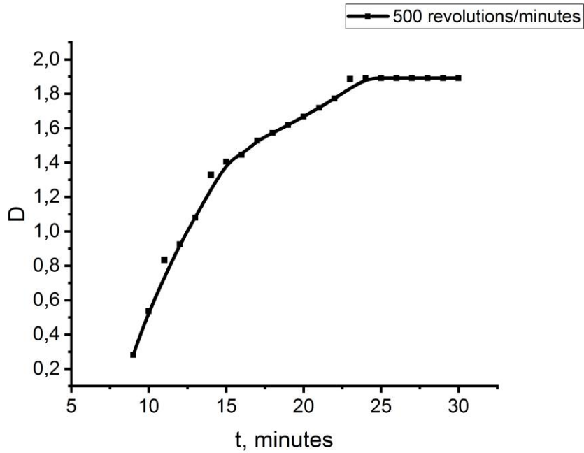
Fig. 2. Dependence of the optical density of the samples on the centrifugation time for centrifugation frequency of 500 rpm.
