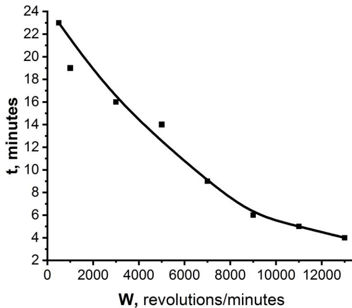
Fig. 3. Dependence of the deposition time of the particles on the rotation speed of the centrifuge.
