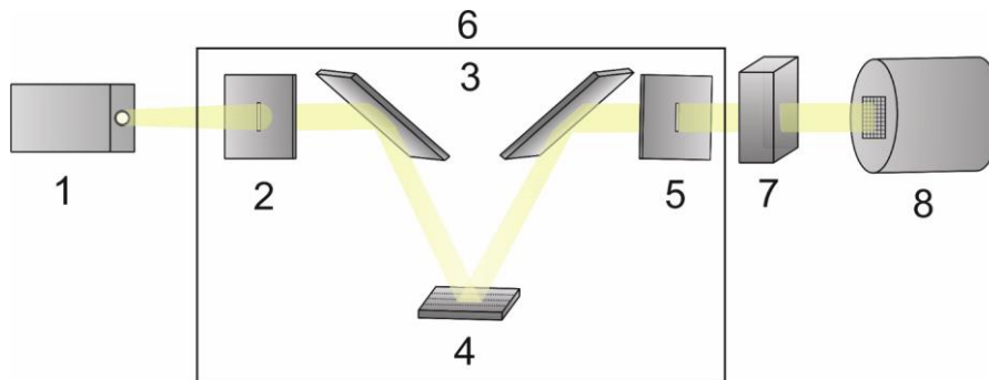
Fig. 1. Setup for measuring the optical density of the samples:
